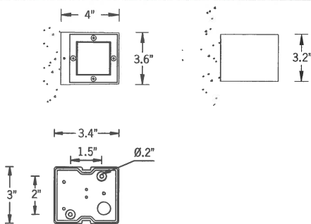
Mounting Detail
