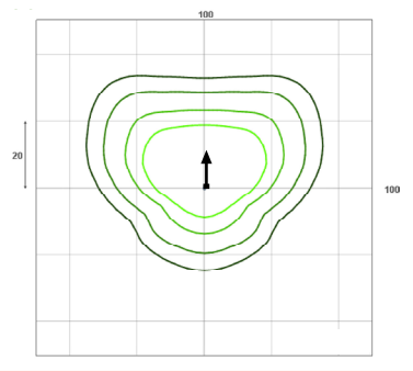
WPX3 LED
