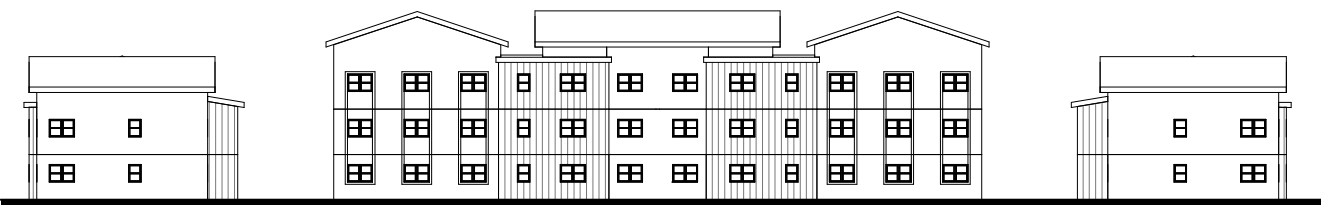
BUILDINGS A, B & C - NORTH ELEVATION (FROM 11TH STREET) 1" = 10'-0"
