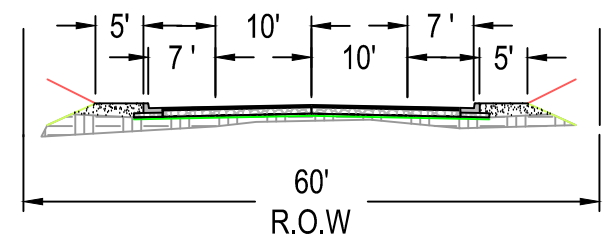
STANDARD SECTION NOT TO SCALE
