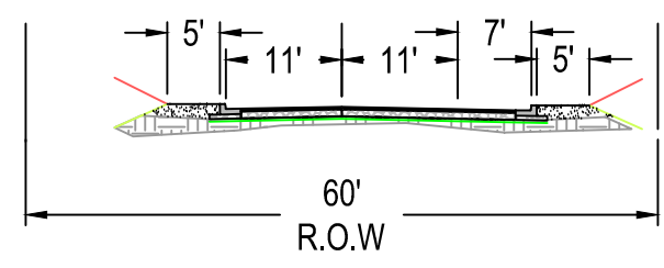
MINIMIZED SECTION W/PARKING NOT TO SCALE
