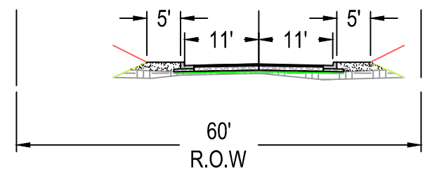
MINIMIZED SECTION NOT TO SCALE
